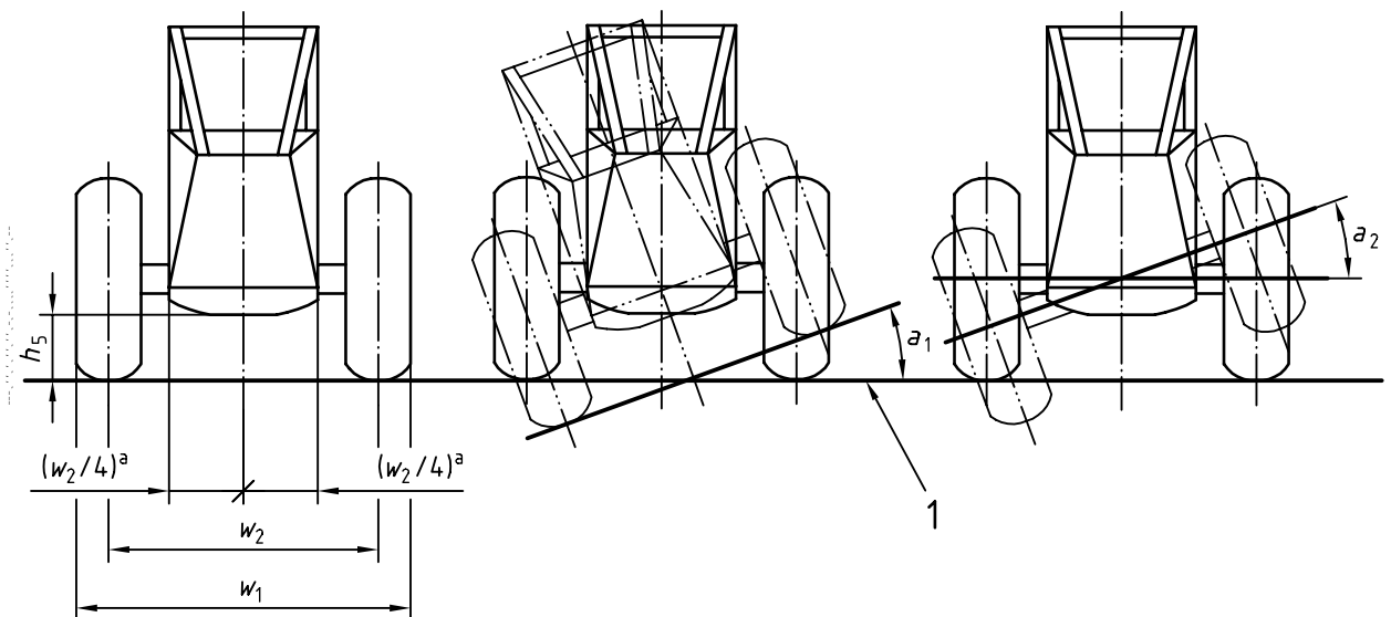
Figure 1 — Articulated rubber-tired skidder
