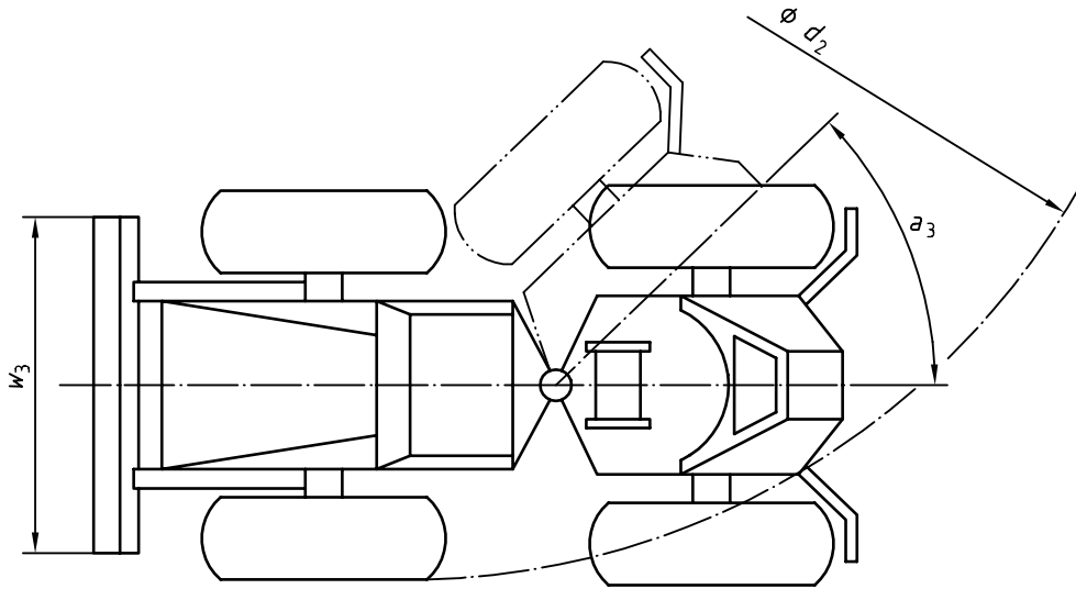
Figure 3 — Steering
