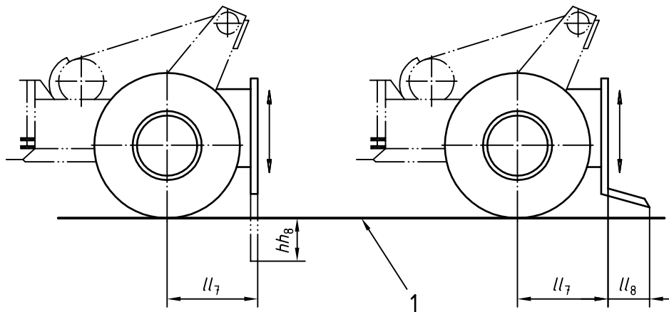
Figure 5 — Grapple specifications
