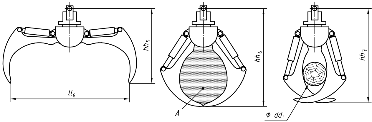
Figure 5 — Grapple specifications
