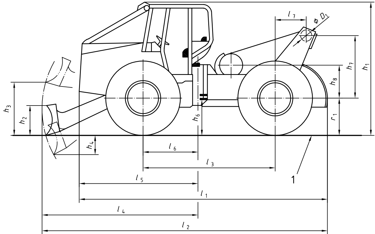
Figure 1 — Articulated rubber-tired skidder
